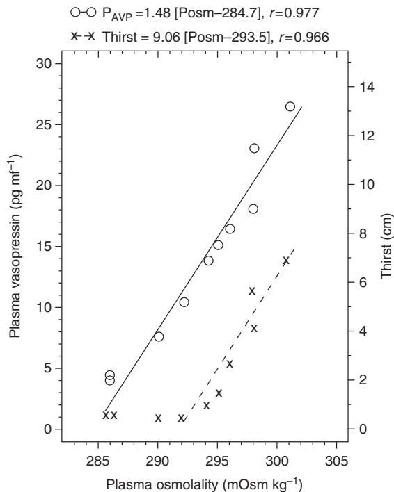
Figure 7 The relationship of plasma vasopressin ( \circ ) and thirst ( \times ) with plasma osmolality in a volunteer during an infusion of 5% saline. Reproduced from Robertson GL (1984) Abnormalities of thirst regulation (Nephrology forum). Kidney International 25: 460–469.
