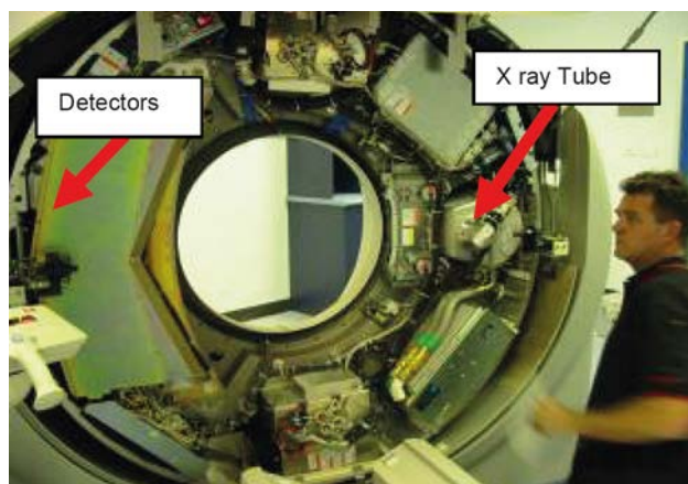
FIG. 2. CT scanner with gantry cover removed. Note the X ray tube on the right hand side with collimator and filters facing towards the scan aperture. Detectors are on the left hand side.
