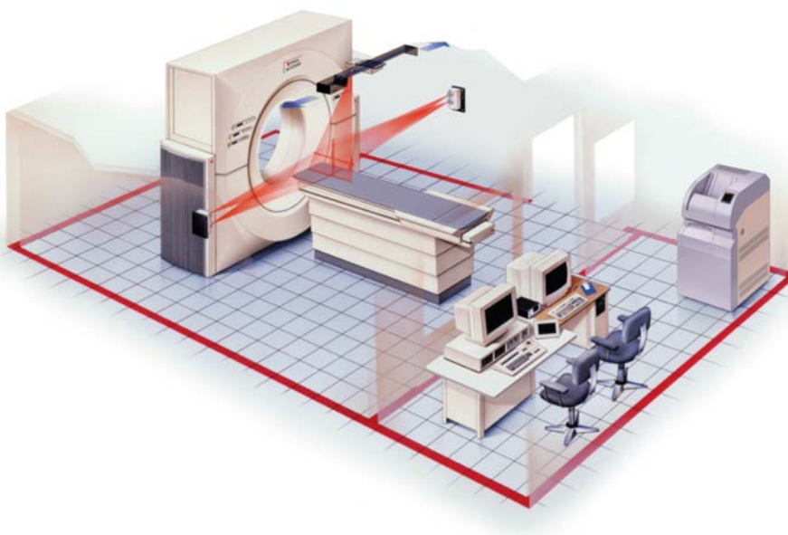
FIG. 7. CT simulator equipped with a flat couch top, external patient positioning/marking system and movable lasers (a) and fixed wall lasers (b) and specialized CT simulation software. (Courtesy: Philips Medical Systems.)
