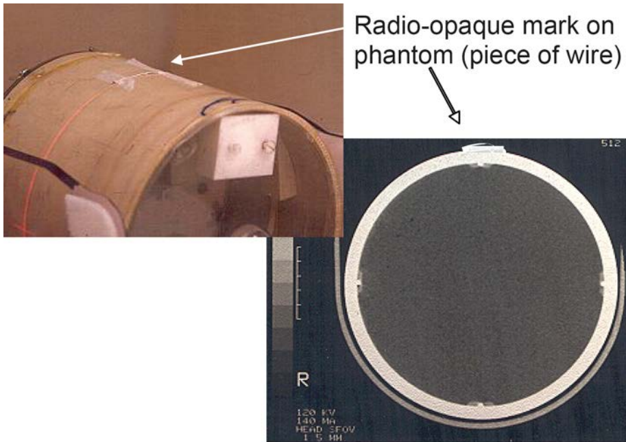
FIG. 20. Light alignment with scan plane: Imaging method.
