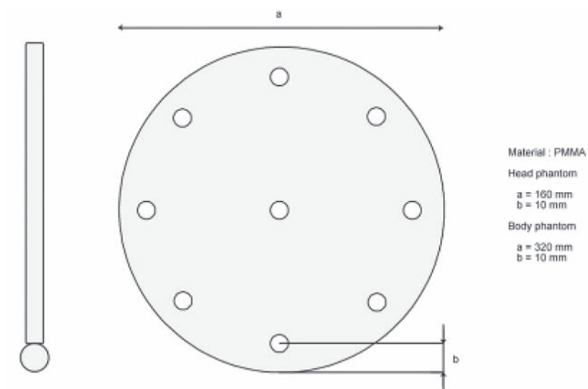
FIG. 38. Cross-section through the standard phantom (head and body dimensions given). The small circles indicate the positions of the bores for inserting a CT ionization chamber. A PMMA plug is shown on the left (not to scale) (from Ref. [26]).
