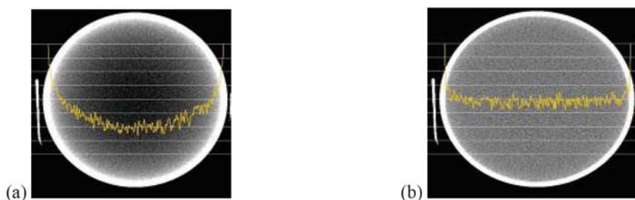
FIG. 10. Example of (a) beam hardening artefact through a water filled phantom and (b) after beam hardening correction applied.
