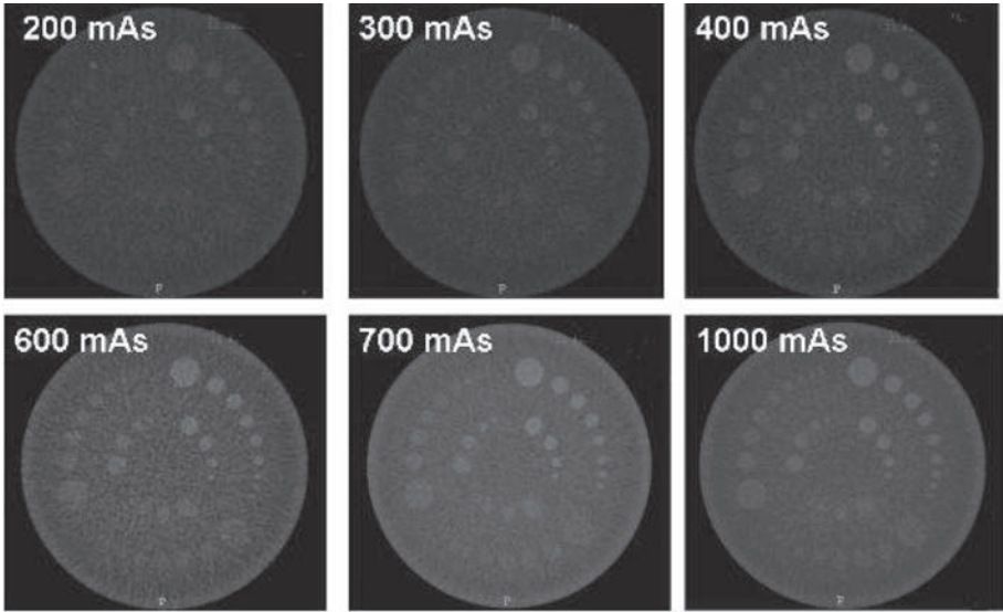
FIG. 18. The effect of mAs on noise and the consequent effect of low contrast visibility.
