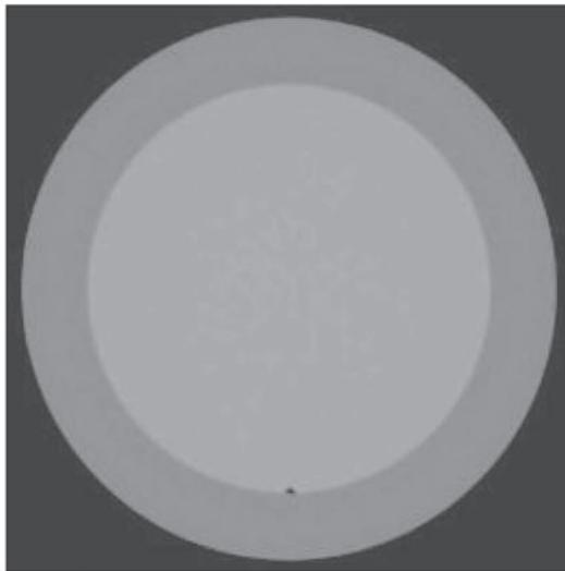
FIG. 31. Noise and uniformity phantom consisting of uniform plastic core and surrounding plastic ring.
