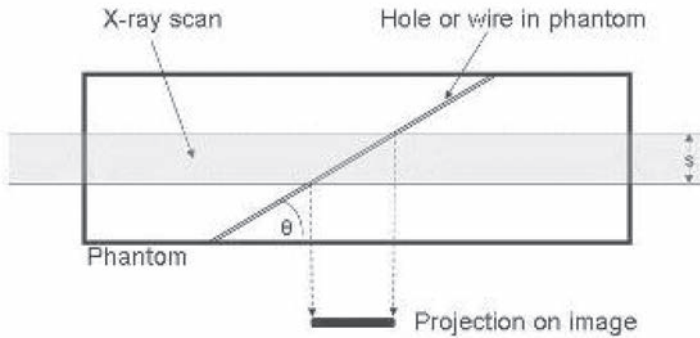
FIG. 34. View of slice width phantom with superimposed CT slice projection and resulting test object projection on image.
