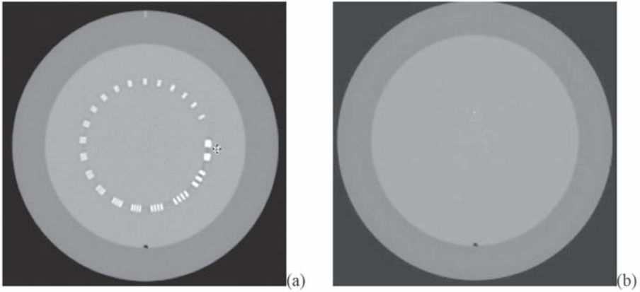
FIG. 33. (a) Line pair high contrast phantom, (b) MTF based high contrast phantom.
