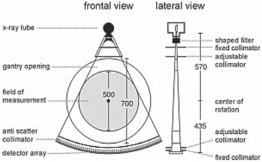
FIG. 3. Schematic representation of the scanning geometry and important components of the CT measurement system in frontal view ( x - y plane) and in lateral view ( y - z plane). (Adapted from Ref. [9] with permission.)
