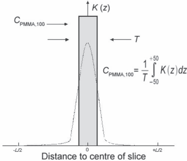
FIG. 13. Profile of air kerma, K(z) measured in the standard CT dosimetry phantom along an axis parallel to the CT scanner axis ( z ) for a single CT slice of nominal width T mm. The CT air kerma index, C_{\text{PMMA},100} is obtained by integrating the air kerma over a length ( L ) of 100 mm (reproduced from Ref. [26]).
