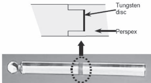
FIG. 35. A typical helical z sensitivity phantom (courtesy: ImPACT) [140].
