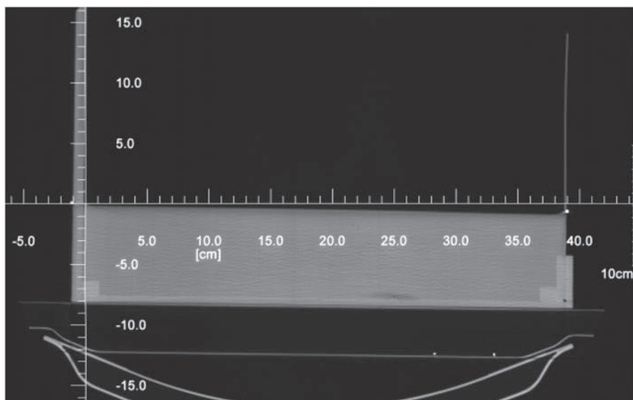
FIG. 28. CT image of a water bath demonstrating a sloping water surface. This indicates that the entire image is rotated.
