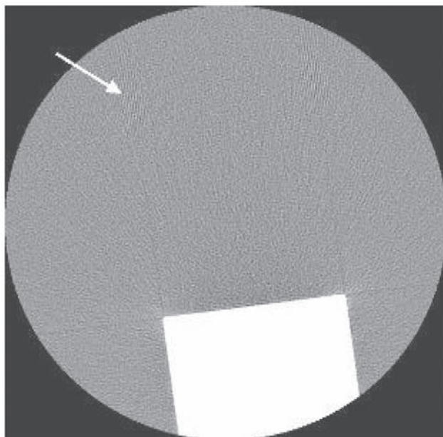
FIG. 12. Example of aliasing artefact.
