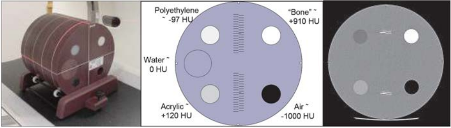
FIG. 41. CT number regions in RMI ACR accreditation phantom.
