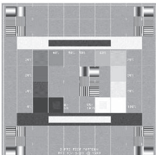
FIG. 22. SMPTE test pattern. Note the 5% and 95% patches inset within the 0% and 100% patches, respectively. These should be visible on the image displays and on the film images. Note that the 0% patch usually cannot be visualized on a printed (reflective) image such as this figure, but should be visible on CT films and displays.
