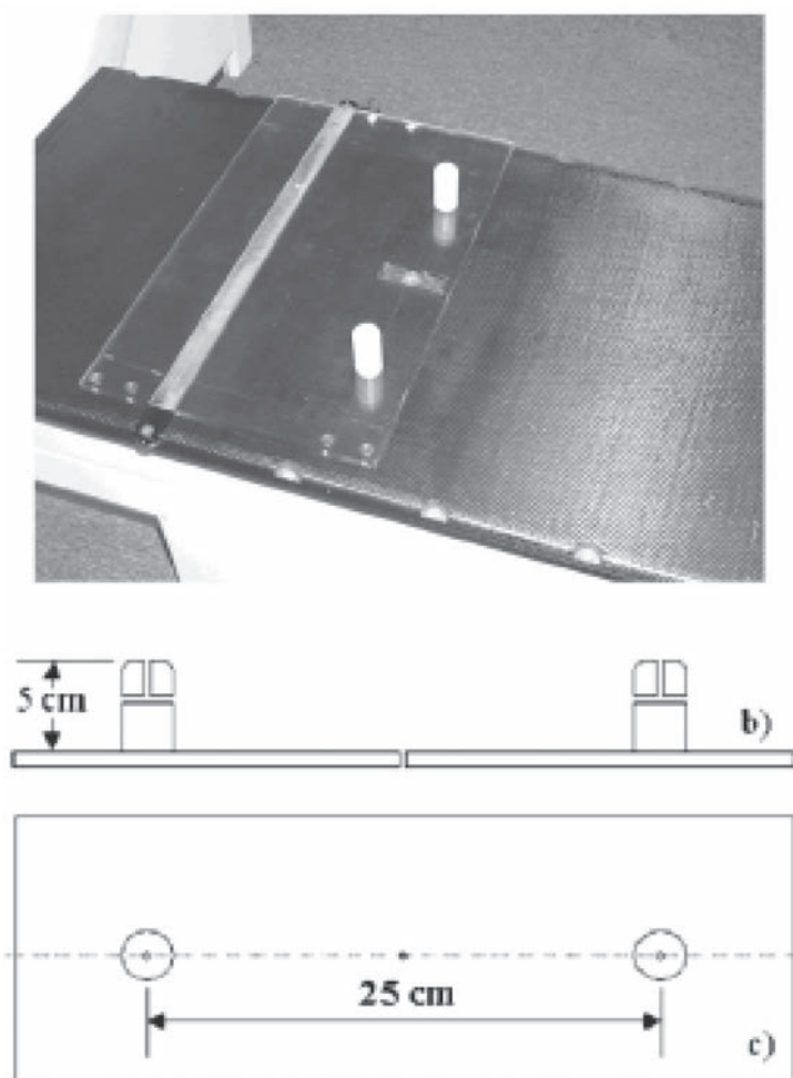
FIG. 36. CT laser QC test tool. (a) CT laser QC device attached to the couch top, (b) side elevation of CT laser device through the centre of the pegs showing holes drilled inside the pegs and (c) plan view of the device (adapted from Ref. [2]).
