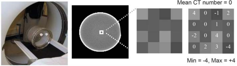
FIG. 8. Variation in grey level from a water phantom (CT number).
