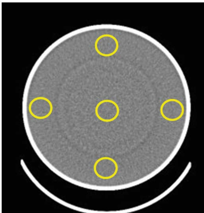
FIG. 24. Placement of ROIs for noise and uniformity measurements. Central ROI used for noise; peripheral and central ROIs for uniformity.
