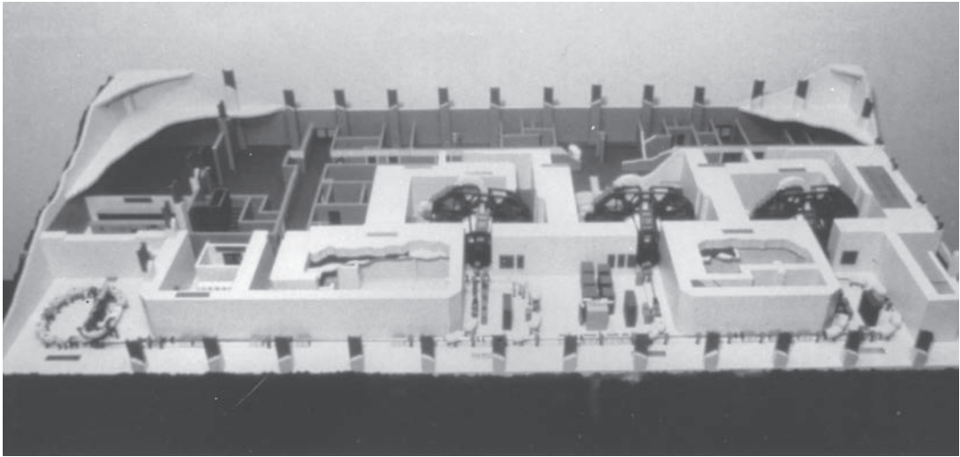
FIGURE 25.5 Model of the proton facility at Loma Linda. Protons are accelerated to energies up to 250 MeV in a large cyclotron. The protons then can be directed into any one of four treatment rooms. This arrangement minimizes “idle” time, because while one patient is being treated in one room, the next two patients can be set up in adjoining treatment rooms. This sort of facility sets the scene for the future: a large radiation therapy facility with multiple treatment rooms in the context of a cancer center. (Courtesy of Drs. James Slater and John Archambeau, Loma Linda University, Loma Linda, California.)
