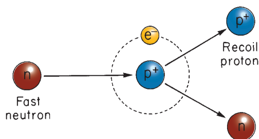
FIGURE 1.9 Interaction of a fast neutron with the nucleus of a hydrogen atom of the absorbing material. Part of the energy of the neutron is given to the proton as kinetic energy. The neutron, deflected from its original direction, proceeds with reduced energy.
