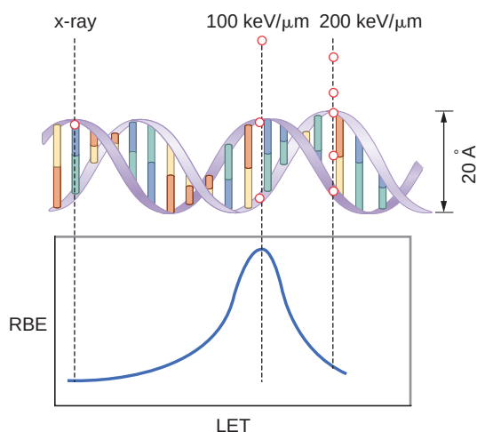
FIGURE 7.6 Diagram illustrating why radiation with a linear energy transfer (LET) of 100 \text{ keV}/\mu\text{m} has the greatest relative biologic effectiveness (RBE) for cell killing, mutagenesis, or oncogenic transformation. For this transfer, the average separation between ionizing events coincides with the diameter of the DNA double helix (i.e., about 20 \text{ \AA} or 2 \text{ nm} ). Radiation of this quality is most likely to produce a double-strand break from one track for a given absorbed dose.
